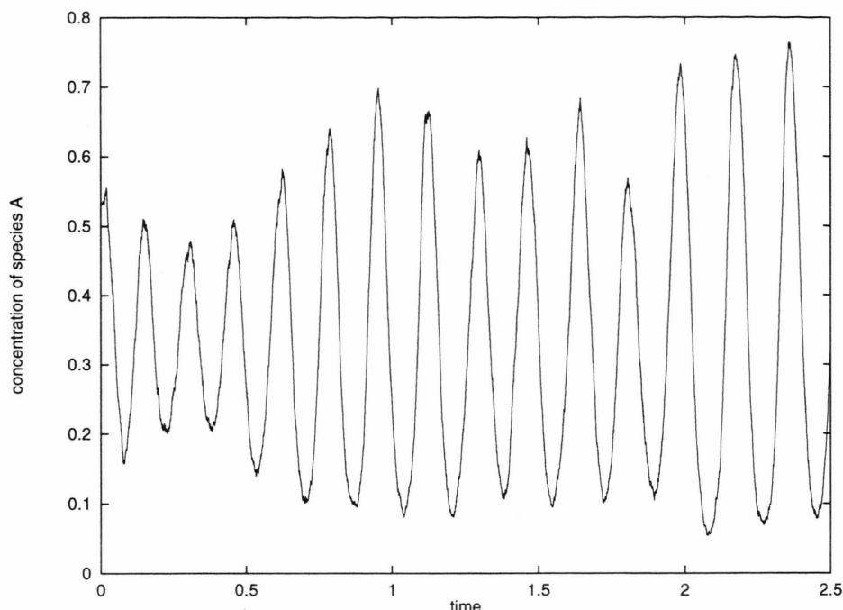
Fig. 1. Concentration of species A as a function of time in the reaction scheme (1), simulated in a plane using 1024 smoothly repulsive point particles. Initial conditions (macroscopic): A(0) = 496/1024 , B(0) = 204/1024 , C(0) = 324/1024 . The concentrations of B and C showed a very similar behavior (displaced by a third of a period). Simulation performed on an Indigo workstation. For details about the Hamiltonian and the algorithm, cf. text.
